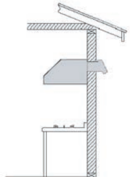
REAR VENTING
